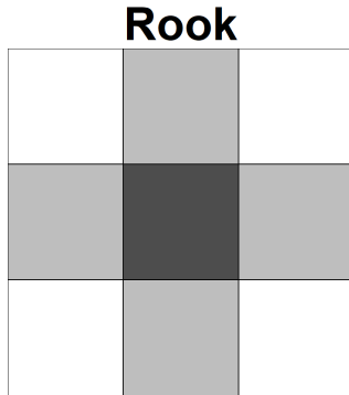
Figure 1: Rook neighbors (light) share an edge with a reference spatial region (dark)[31]
